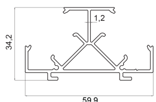
Profil LED
